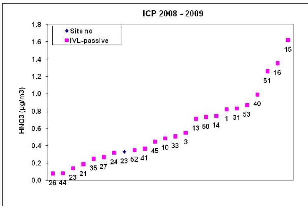
Figure 4: The spread in the yearly mean \text{HNO}_3 values for the test sites for the test period for ICP Materials.
